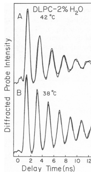
FIGURE 2 The diffracted probe intensity as a function of probe delay time in the liquid crystal phase (A) and gel phase (B) of 280- \mu\text{m} thick aligned DLPC multibilayers containing 2% water by weight. The phase transition temperature T_c is 40 ^{\circ}\text{C} . Also shown is the least-squares fit of the data to Eq. 1, which yields the acoustic velocity V and attenuation \alpha . In A, V = 1.82 \times 10^5 cm/s and \alpha/f^2 = 560 \times 10^{-17} s ^2 /cm. In B, V = 1.97 \times 10^5 cm/s and \alpha/f^2 = 280 \times 10^{-17} s ^2 /cm.
